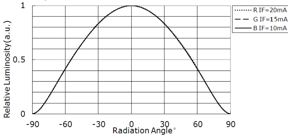
Directivity X-X
