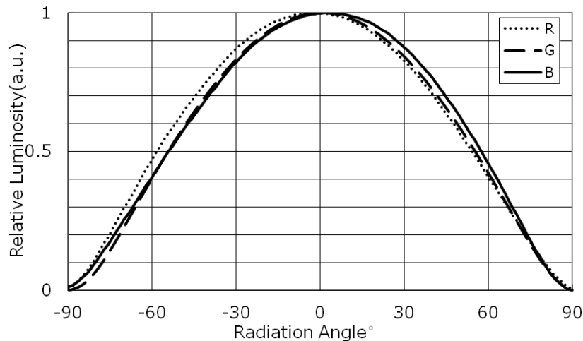
Directivity Y-Y
