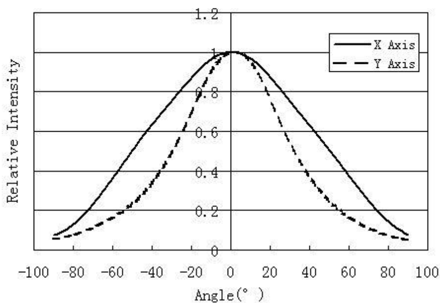
Radiation patterns
