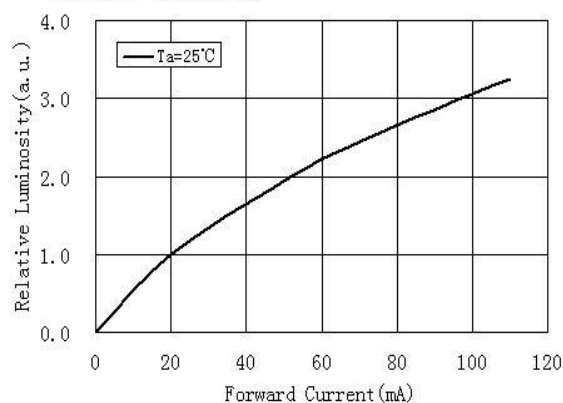
Forward Current vs. Relative Luminosity
