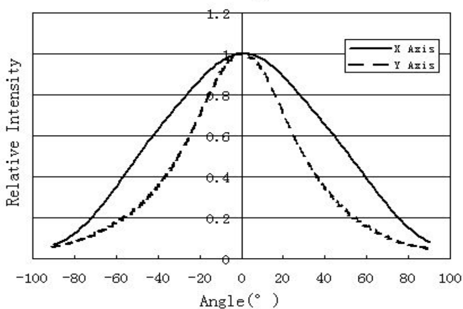
Radiation patterns
